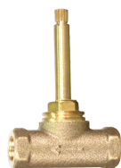
KB111007 Concealed Stop Cock Body- G1/2" (15 mm)
