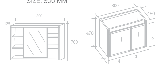
KAJ0520 CARBON FIBER SIZE: 800 MM
