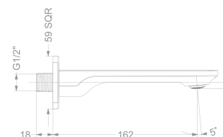
KB2911016-CP / RG / CG / GM / MBK BATH SPOUT WITH FLANGE
