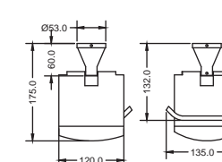
KA700009-MBK TOILET PAPER HOLDER WITH FLAP
