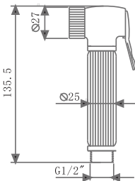
KA580011-CGL HEALTH FAUCET (BRASS) WITH HOOK & 1 M HOSE
