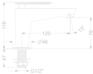
KB2311001-CP / RG / CG / GM / MBK PILLAR TAP
