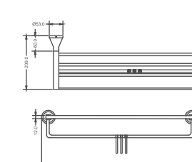
KA700010-MBK TOWEL RACK WITH HOOK 24"
