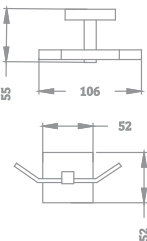
KA990003-CRG / CGL / RG / GM TWIN ROBE HOOK
