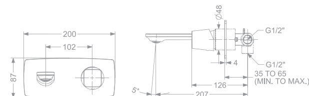
KB2911023-CP / RG / CG / GM / MBK CONCEALED WALL MOUNTED SINGLE LEVER BASIN MIXER TRIMS (COMPATIBLE WITH KB2911022-CP / RG / CG / GM / MBK)
