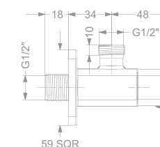
KB2911003-CP / RG / CG / GM / MBK ANGLE VALVE WITH FLANGE
