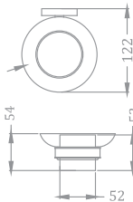
KA990004-CRG / CGL / RG / GM SOAP DISH
