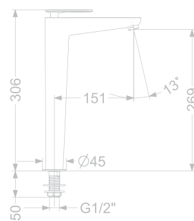
KB2311002-CP / RG / CG / GM / MBK TALL PILLAR TAP
