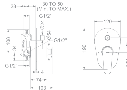
KB2311037-CP / RG / CG / GM / MBK 2 INLET HI-FLOW CONCEALED SINGLE LEVER DIVERTER TRIMS (COMPATIBLE WITH KB911035-CP / RG / CG / GM / MBK)
