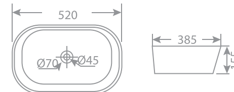
KAJ0455-GR GLOSSY GOLD RIM & WHITE WASH BASIN (COMPATIBLE POP-UP KAJ0528-MW)
