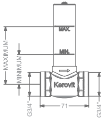
KB111061 CONCEALED STOP COCK BODY (Heavy) - G3/4" (20MM)
