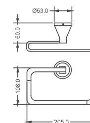
KA700005-MBK TOWEL HANGER
