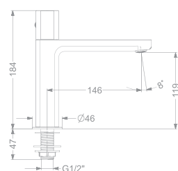
KB2911001-CP / RG / CG / GM / MBK PILLAR TAP
