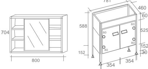
KAJ0550 CARBON FIBER SIZE: 800 MM
