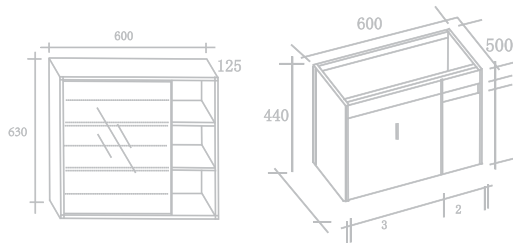
KAJ0522-S CARBON FIBER SIZE: 600 MM
