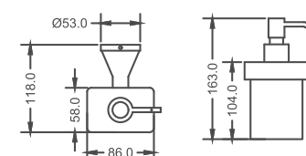
KA700015-MBK SOAP DISPENSER
