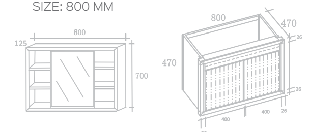
KAJ0519 CARBON FIBER SIZE: 800 MM
