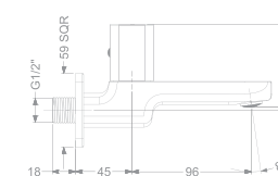
KB2911004-CP / RG / CG / GM / MBK BIB TAP WITH FLANGE
