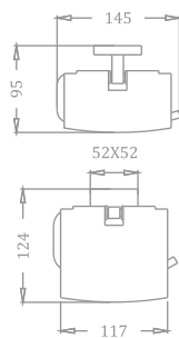
KA990009-CRG / CGL / RG / GM TOILET PAPER HOLDER WITH FLAP
