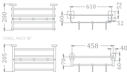
KA990010 / 11-CRG / CGL / RG / GM TOWEL RACK WITH HOOK 24" / 18"
