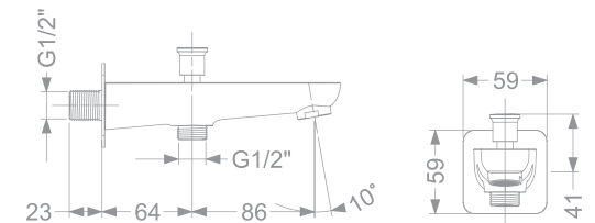
KB2311017-CP / RG / CG / GM / MBK BATH TUB SPOUT WITH DIVERTER & FLANGE
