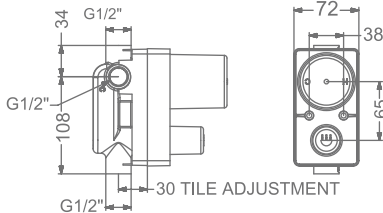
CONCEALED HI-FLOW DIVERTER BODY- SL
