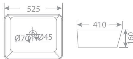
KAJ0456-GR GLOSSY GOLD RIM & WHITE WASH BASIN (COMPATIBLE POP-UP KAJ0528-MW)
