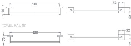
KA990001 / 2-CRG / CGL / RG / GM TOWEL RAIL 24" / 18"
