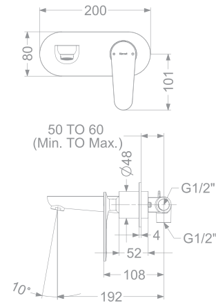
KB2311023-CP / RG / CG / GM / MBK CONCEALED SINGLE LEVER WALL MOUNTED BASIN MIXER TRIMS (COMPATIBLE WITH KB2311022-CP / RG / CG / GM / MBK)
