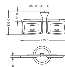
KA700016-MBK DOUBLE SOAP DISH
