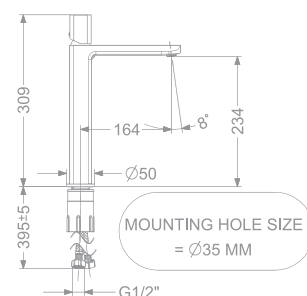
KB2911011-ND-CP / RG / CG / GM / MBK SINGLE LEVER TALL BASIN MIXER WITHOUT POP-UP
