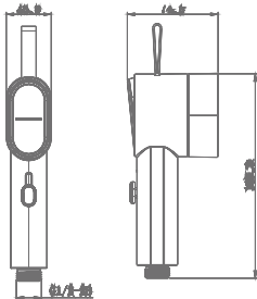
KA580024-MB / MG / MW 2 FLOW HEALTH FAUCET WITH HOOK & 1 M HOSE
