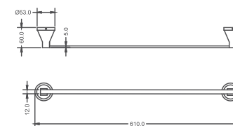
KA700001-MBK TOWEL RAIL 24"
