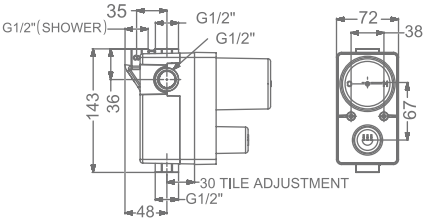
CONCEALED 3 INLET DIVERTER BODY- SL
