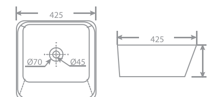
KAJ0454-GR GLOSSY GOLD RIM & WHITE WASH BASIN (COMPATIBLE POP-UP KAJ0528-MW)
