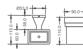
KA700007-MBK TUMBLER HOLDER
