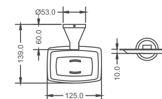
KA700004-MBK SOAP DISH
