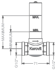
KB111060 CONCEALED STOP COCK BODY (Heavy) - G1/2" (15MM)
