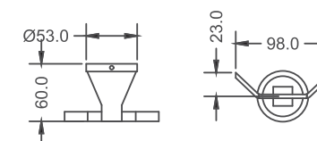
KA700003-MBK TWIN ROBE HOOK
