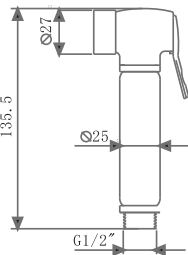
KA580023-CP / RG / CG / GM HEALTH FAUCET (BRASS) WITH HOOK & 1 M HOSE
