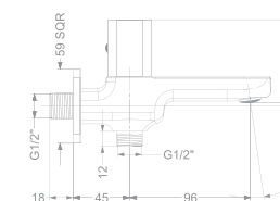
KB2911005-CP / RG / CG / GM / MBK 2 WAY BIB TAP WITH FLANGE
