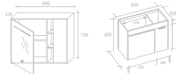
KAJ0523 CARBON FIBER SIZE: 800 MM
