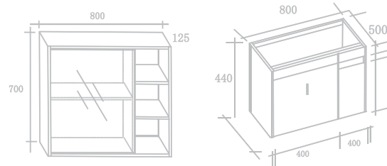
KAJ0522 CARBON FIBER SIZE: 800 MM
