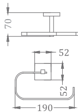
KA990005-CRG / CGL / RG / GM TOWEL HANGER
