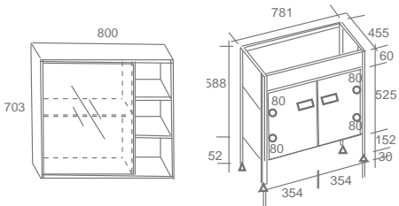
KAJ0553 CARBON FIBER SIZE: 800 MM
