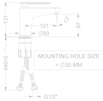
KB2311010-ND-CP / RG / CG / GM / MBK SINGLE LEVER BASIN MIXER WITHOUT POP-UP
