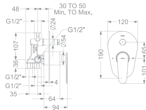
KB2311036-CP / RG / CG / GM / MBK 3 INLET CONCEALED SINGLE LEVER BATH & SHOWER MIXER TRIMS (COMPATIBLE WITH KB2311034-CP)
