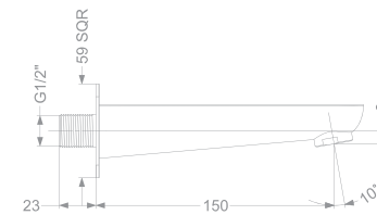
KB2311016-CP / RG / CG / GM / MBK BATH SPOUT WITH FLANGE
