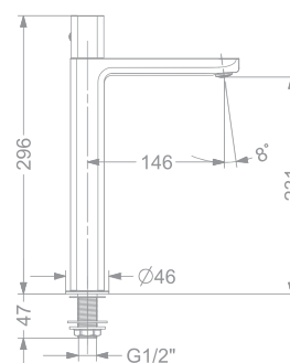
KB2911002-CP / RG / CG / GM / MBK TALL PILLAR TAP
