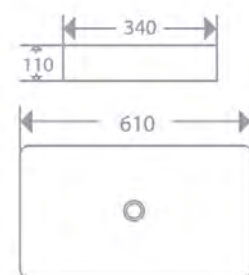
KAJ0491 MATTE LIGHT GREEN WASH BASIN (COMPATIBLE POP-UP KAJ0527-LGR)
