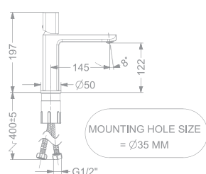
KB2911010-ND-CP / RG / CG / GM / MBK SINGLE LEVER BASIN MIXER WITHOUT POP-UP
