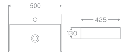
KAJ0364-MW / KAJ0377-MB POSH, THIN RIM WASH BASIN (COMPATIBLE POP-UP KAJ0528-MW/MB) SIZE: 500x425x130 MM
