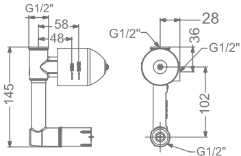
CONCEALED WALL MOUNTED BASIN MIXER BODY- SL
